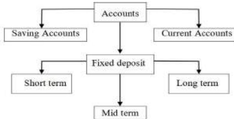
Figure 9.3: Hierarchical Inheritance
