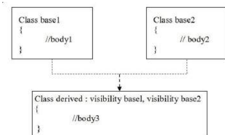
Figure 9.2: Multiple Inheritance
